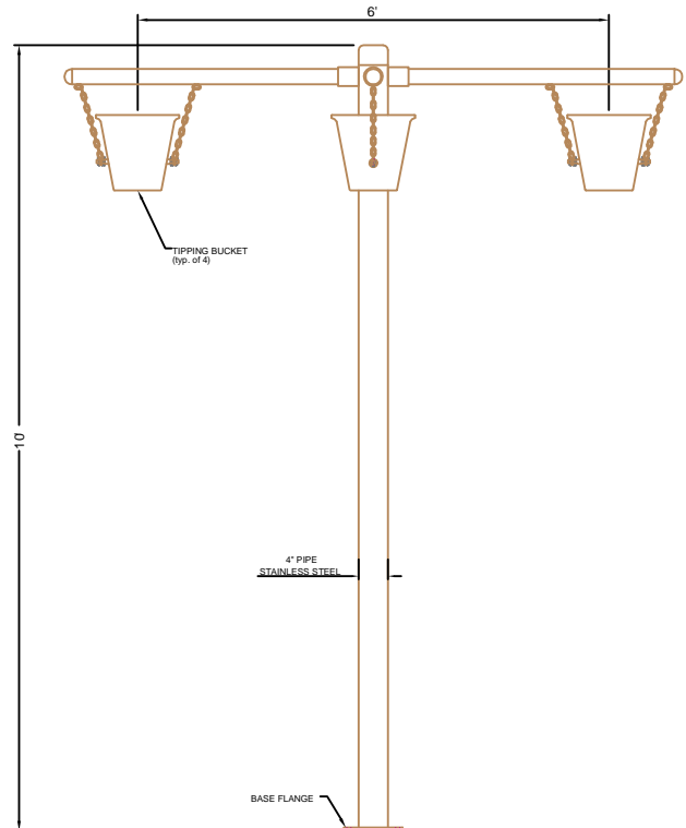
ELEVATION VIEW
