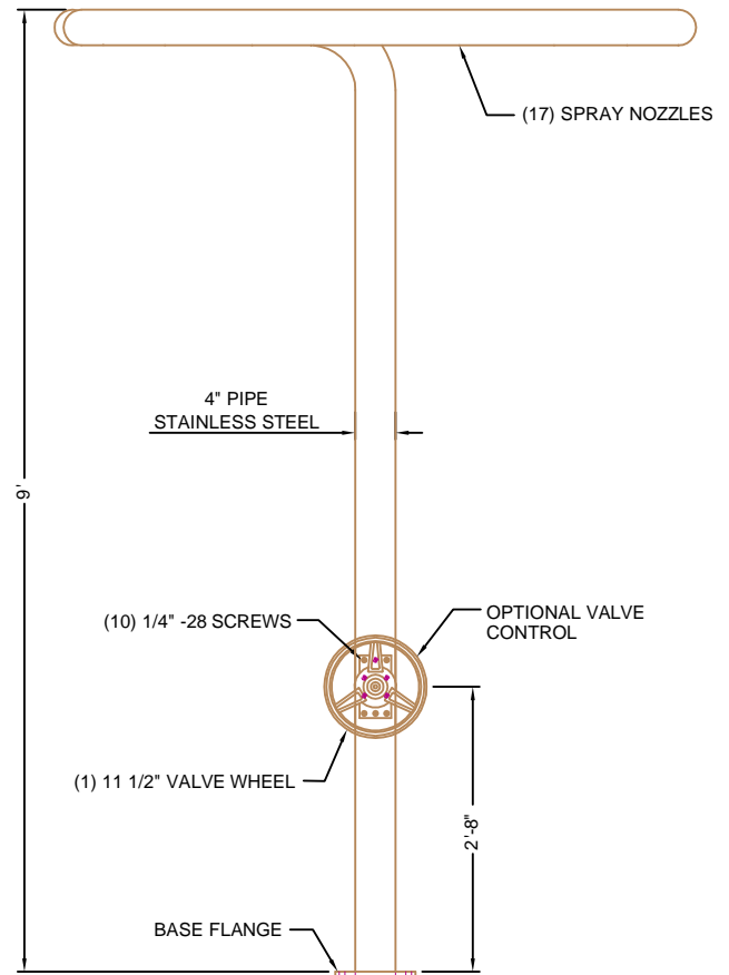
ELEVATION VIEW
