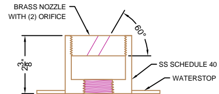
ELEVATION VIEW
