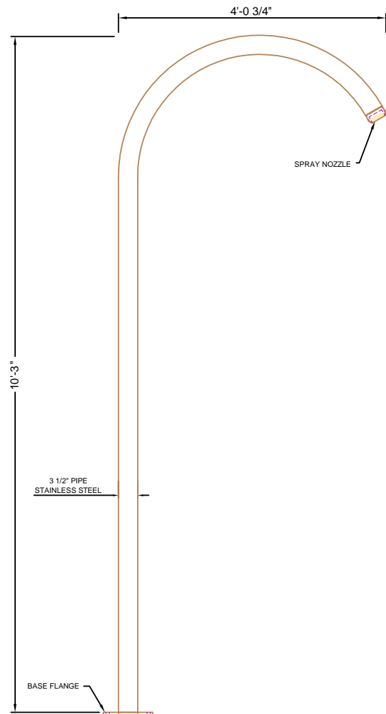
ELEVATION VIEW
