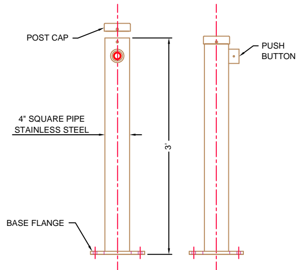
ELEVATION VIEW
